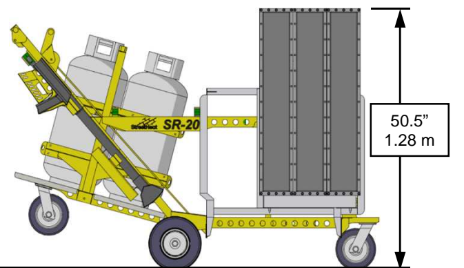
Dimensions with Heater Bank Folded
