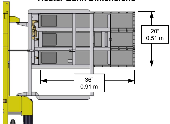
Heater Bank Dimensions
